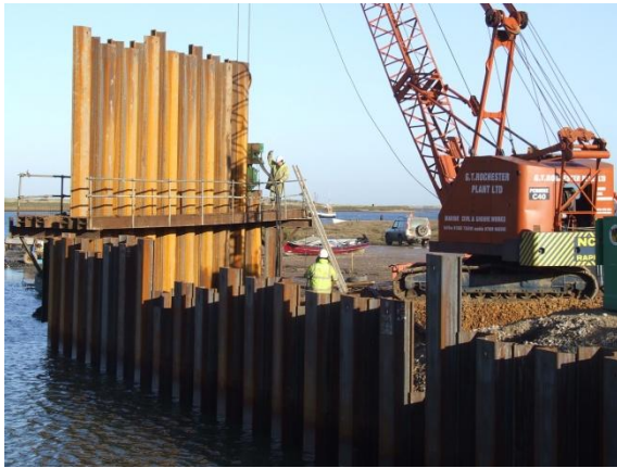
Installing sheet piled wall
